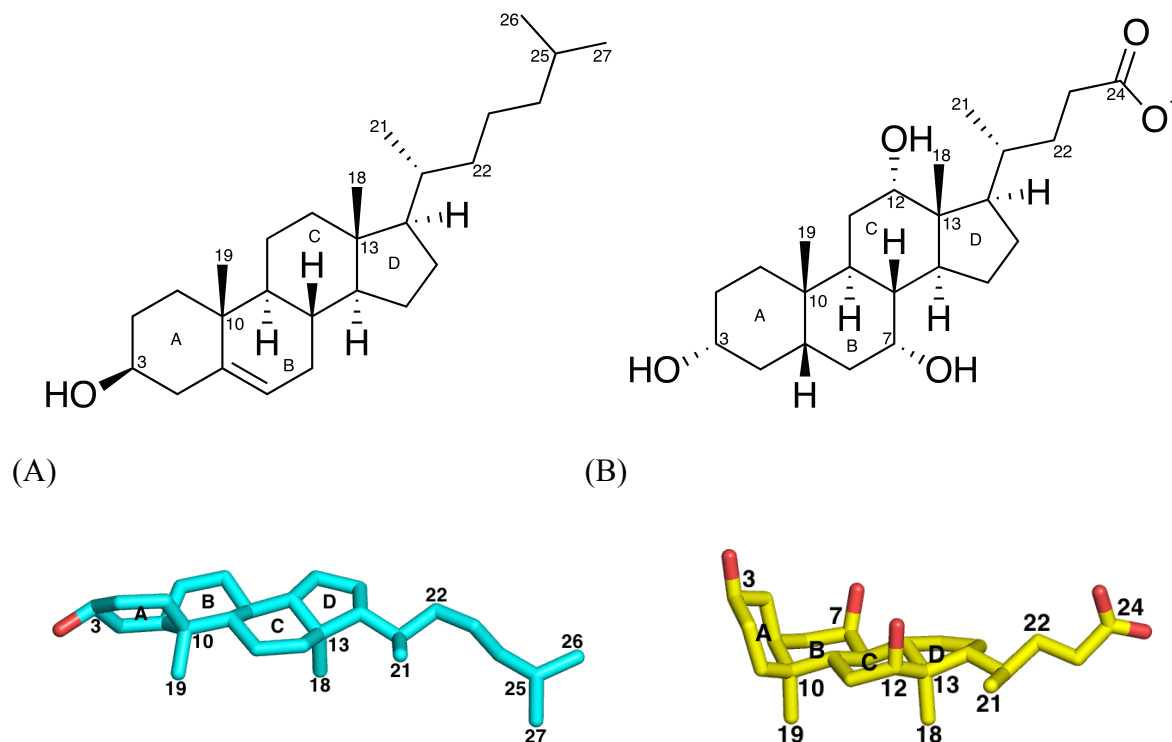
Figure 1. 2D and 3D chemical structures of (A) cholesterol (blue) and (B) cholate (yellow), with the flexible tails from C21 to C24/C25 shown in arbitrary favorable conformations.
