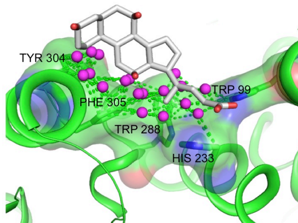
Figure 7. Conserved interaction points for CholMine cholate site prediction (purple spheres) are shown in the context of the interactions between the representative membrane protein query site 2DYR_CHD525C from cytochrome c oxidase, and its bound cholate molecule (white tubes with oxygen atoms in red). Essential residues contributing to the conserved interaction are labeled.
