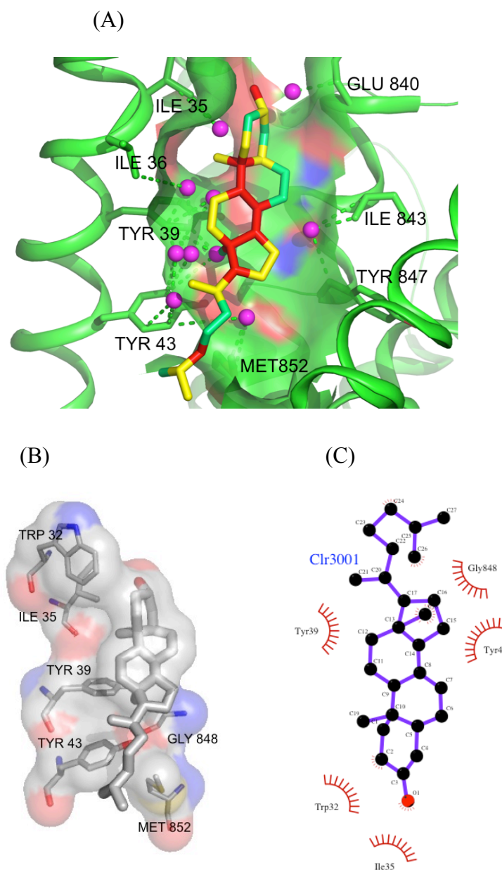
Figure 6. (A) Sodium/potassium-transporting ATPase cholesterol site (PDB entry 3KDP, residue D3001) used as the representative query for CholMine predictions. Purple spheres represent conserved interaction points in the membrane proteins binding cholesterol (from Figure 2), displayed in the context of the representative site from 3KDP. The green dashed lines connect the conserved interaction points to corresponding protein atoms. Cholesterol atoms colored in green contact a protein atom in 60% of the training set sites, atoms colored yellow have a 30-60% frequency of contact, and atoms colored in red contact the protein in <30% of the sites. (B) For comparison, LigPlot + 3-dimensional view (shown with PyMOL; Schrödinger, New York, NY; http://pymol.org ) of key sodium/potassium-transporting ATPase cholesterol interactions identified in just the single structure of 3KDP. (C) Alternative LigPlot 2-dimensional view of these interactions.
