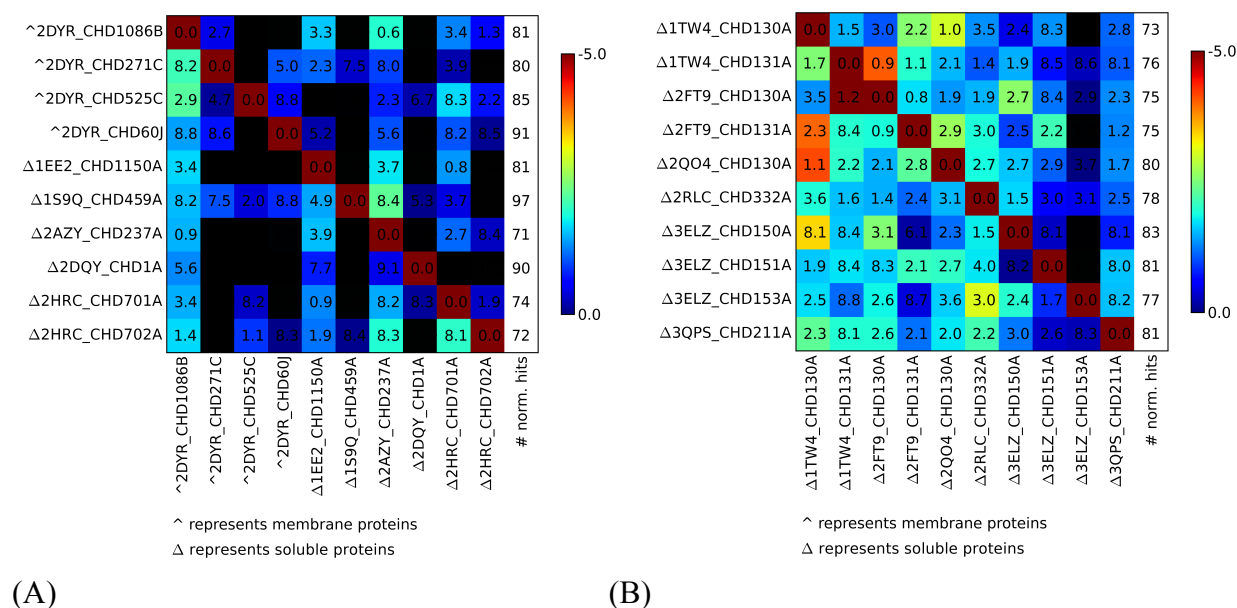
Figure 5. Pairwise alignment and similarity scoring. (A) All-against-all SimSite3D similarity comparison for the first dataset, which includes 4 membrane cholate binding sites and 6 soluble cholate binding sites. (B) All-against-all comparison for the second dataset, which includes another 10 soluble cholate binding sites unrelated to the first set. (See Figure 4 legend for additional details.)
