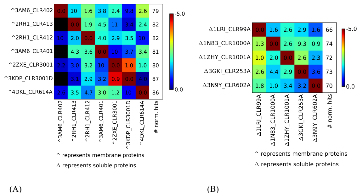
Figure 4. Pairwise alignment and similarity scoring. (A) All-against-all SimSite3D comparison for membrane protein cholesterol binding sites. (B) All-against-all comparison for soluble protein cholesterol binding sites. For the top-scoring alignment of each site pair, the SimSite3D similarity score values are colored from red (most similar) to dark blue (marginally similar) with corresponding score values ranging from -5 to 0 (in standard deviations above the mean score when the same query site is compared to the set of 140 diverse ligand binding sites, where more negative is more significant). Black indicates failure to meet the normalized score threshold of 0. Numbers reported in the grid are the RMSD values (Å) between cholesterol rings following SimSite3D site alignment. Lower RMSD indicates better alignment between sites. The “# norm. hits” column on the right side of each matrix reports the number of sites meeting the scoring threshold for similarity to the query site (labeled to the left in each row) when searching against the 140 sites in the diverse dataset (Table S1), which includes one true positive cholesterol site. The high number of false positives is based on SimSite3D alignment score only, before the conserved interaction points for cholesterol sites have been considered.
