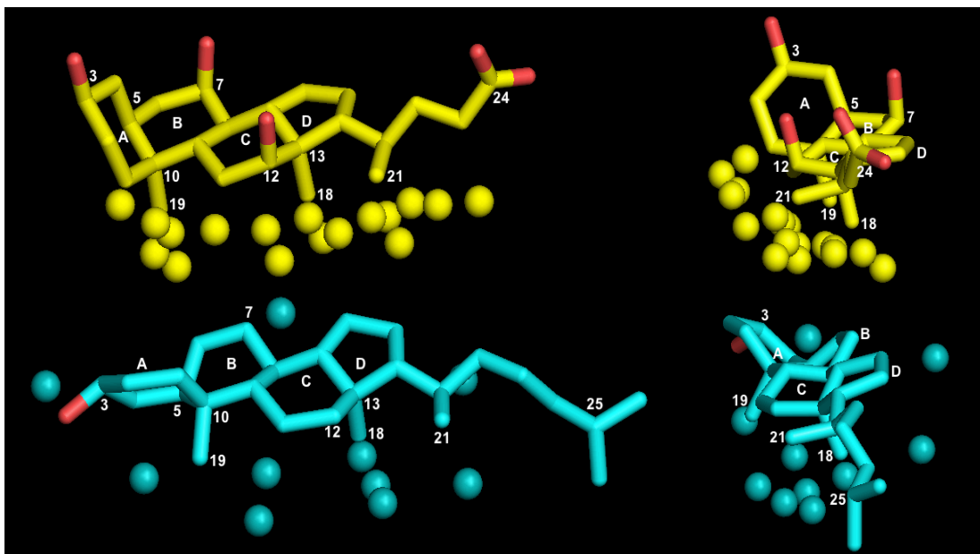
Figure 8. SimSite3D-identified conserved interactions for cholate (yellow) and cholesterol (blue) recognition around along the groove formed between the row of C18, C19, and C21 methyl groups on the beta (lower) face of the steroid and the edge of the steroid ring system. The view on the right is rotated roughly 90 degrees about a vertical axis through the center of each molecule. Cholate sites are distinguished from cholesterol primarily based on interactions with the relatively conserved C22-C23 tail orientation in cholate, and numerous conserved interactions associated with the strongly bent (5-beta configuration) joint between the A and B rings of the cholate steroid ring system. Because the tail configurations are conformationally diverse in different binding sites, conserved interactions are absent in the C24-C25 region.
